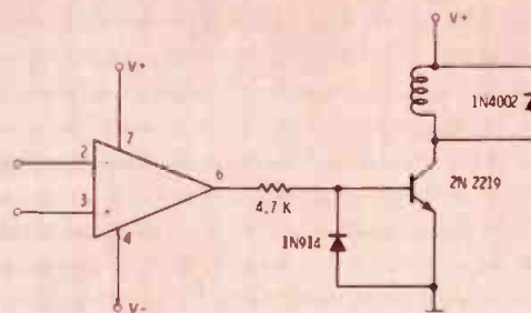
Fig. 2c Comparator driving a relay with power buffer.
