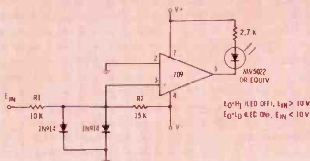
Fig. 2b Comparator driving an LED indicator.
